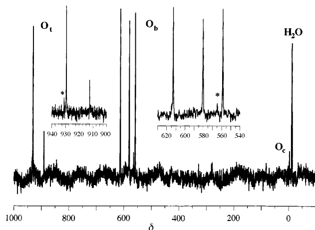
Fig. 4 Natural abundance ^{17}\text{O} NMR spectrum of [n\text{-Bu}_4\text{N}][\text{Mo}_6\text{Cp}^*\text{O}_{18}] in \text{CH}_3\text{CN}-\text{CD}_3\text{CN} , recorded at 343 K. * Represents the [\text{Mo}_6\text{O}_{19}]^{2-} impurity.
