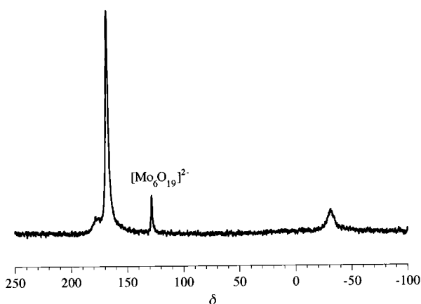
Fig. 3 The ^{95}\text{Mo} NMR spectrum of [n\text{-Bu}_4\text{N}][\text{Mo}_6\text{Cp}^*\text{O}_{18}] in \text{CH}_3\text{CN}-\text{CD}_3\text{CN} , recorded at 343 K.
